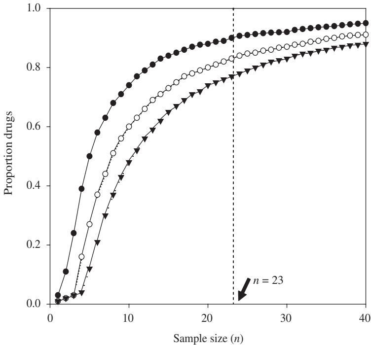
Figure II. Confidence against sample size
