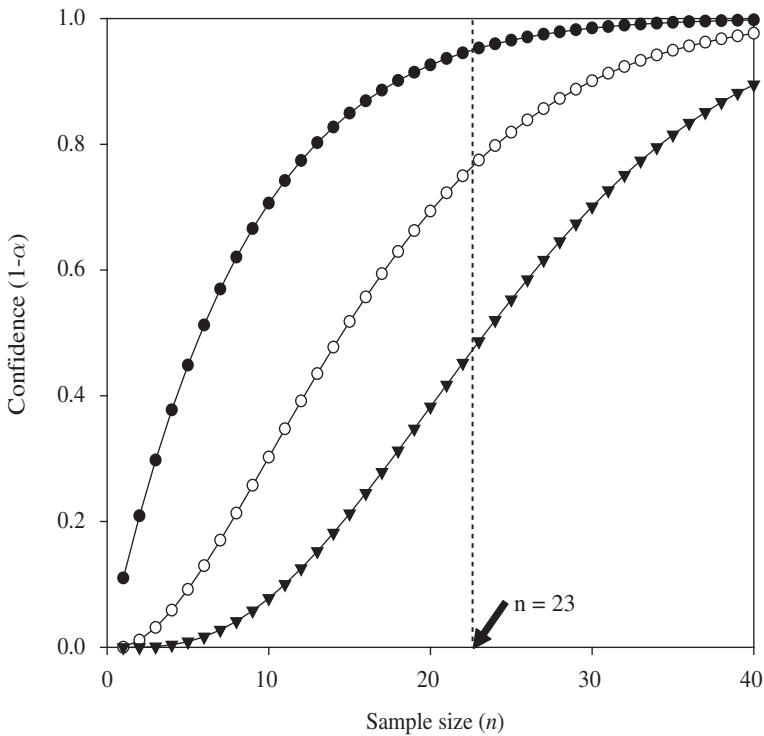
Confidence against sample size ( N = 100 ; k = 0.9 ) for 0, 1, and 2 negatives expected. Lines ● for 0 negatives; ○ for 1 negative; ▼ for 2 negatives.
